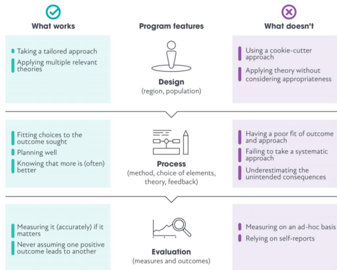
Figure 2 Energy efficiency interventions – What works and what doesn't
